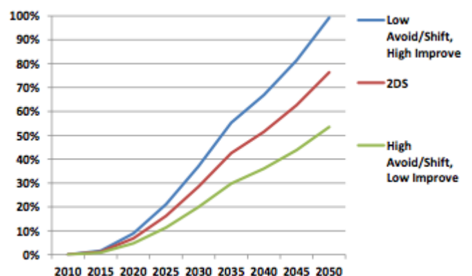
Figures 8. LDV Fuel Carbon Intensity in 2DS and weighted average intensity in all three cases.
